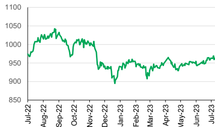
LQ45 (YoY)
