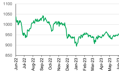
LQ45 (YoY)
